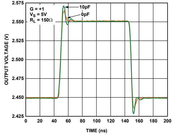
Figure 22. Small Signal Transient Response for Capacitive Load
