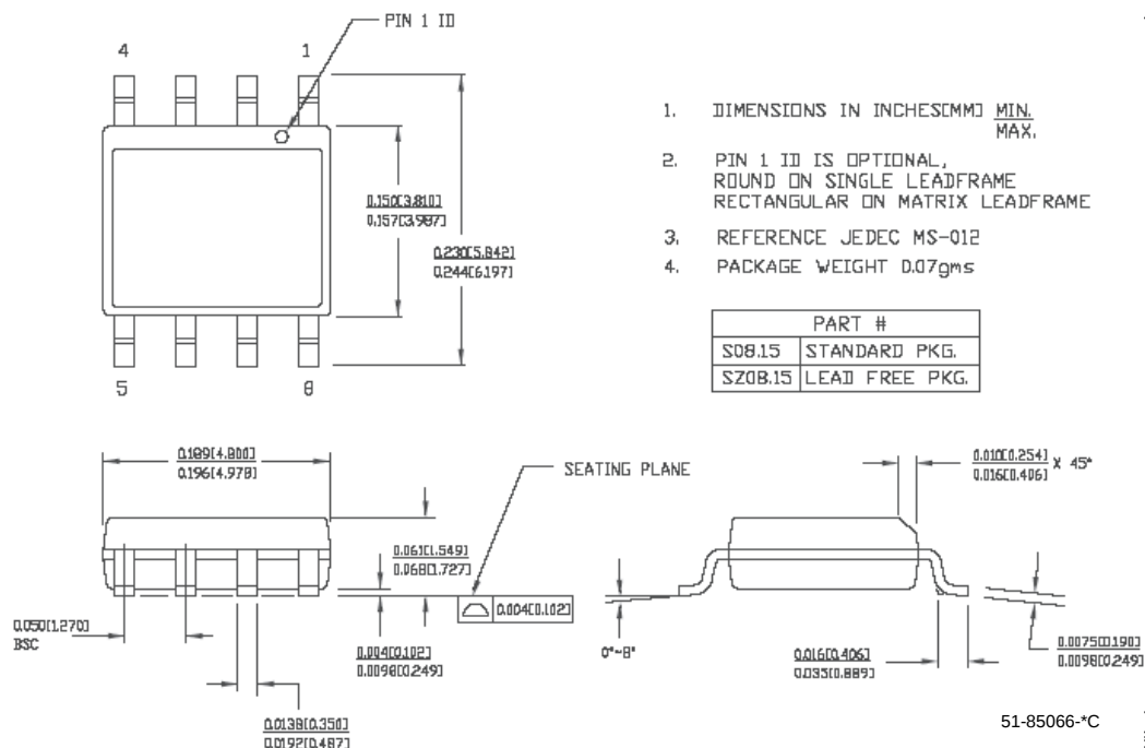
Figure 11-1. 8-Lead (150) SOIC
