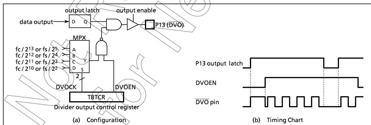
Figure 2-17. Divider Output
