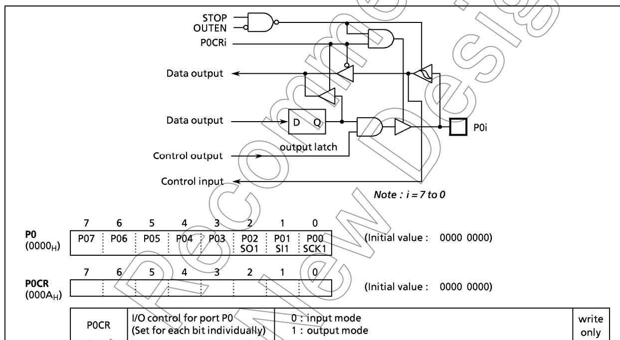
Figure 2-3. Port P0 and P0CR
