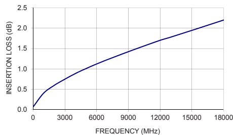
141-40SM+ INSERTION LOSS
