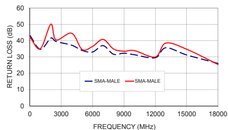
141-40SM+ RETURN LOSS
