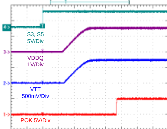
Power On from S3, S5
