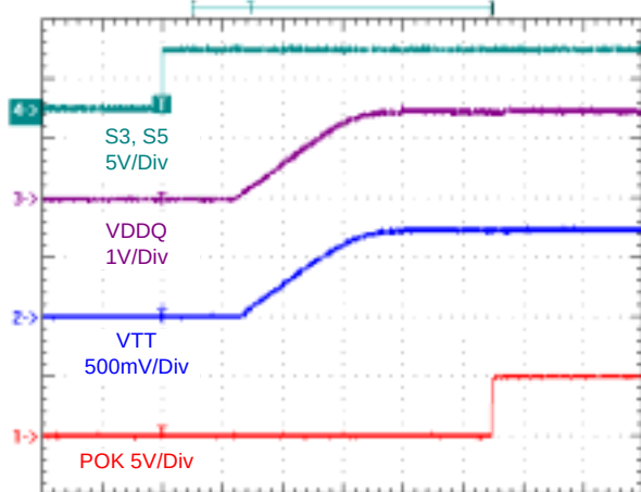
Power On from S3, S5
