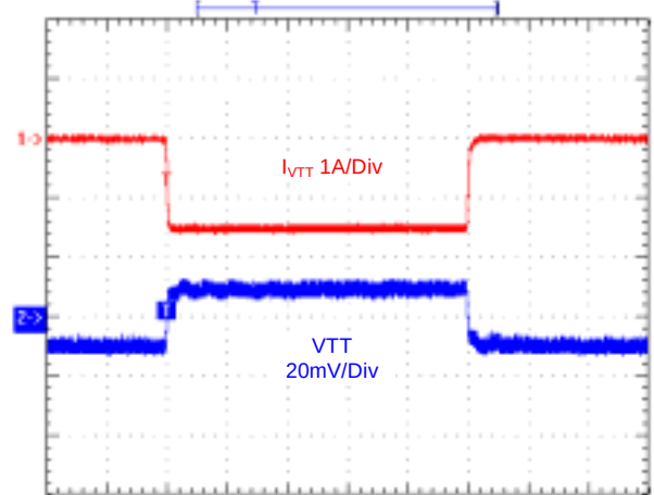
Sink Current: 0A to 1.5A
