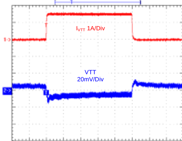
Source Current: 0A to 1.5A
