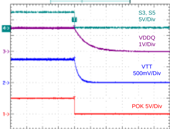
Power Off from S3, S5 with Light Load, Non Tracking Discharge
