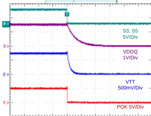
Power Off from S3, S5 with Heavy Load, Non Tracking Discharge
