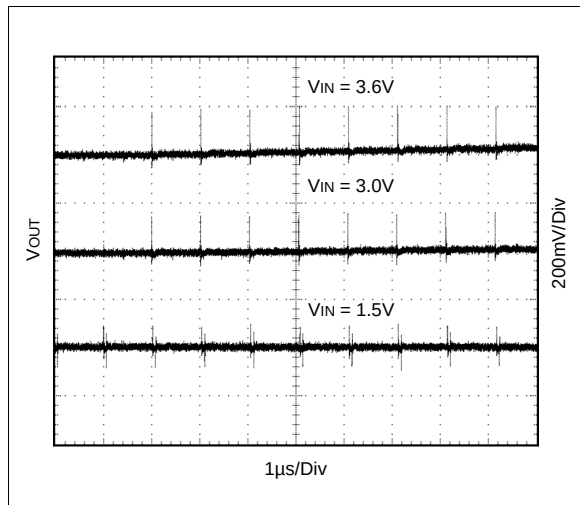
Figure 28. Output Voltage Ripple; V_{OUT} = 18V , I_{OUT} = 1mA
