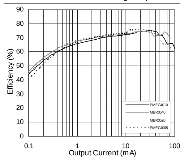
Figure 40. Efficiency Comparison of different Diodes; V_{IN} = 3.6V , V_{OUT} = 18V , L_1 = 6.8\mu H
