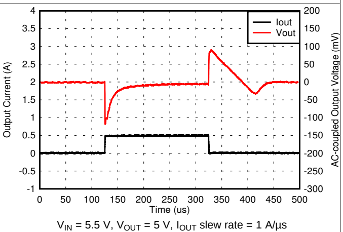
Figure 34. 5-V, 1-mA to 500-mA Load Transient
