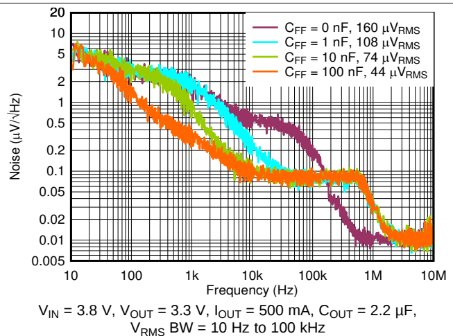
Figure 46. Output Spectral Noise Density vs Frequency and C_{FF}
