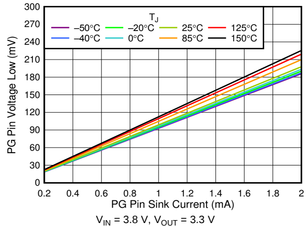
Figure 22. V_{OL(PG)} vs PG Pin Sink Current
