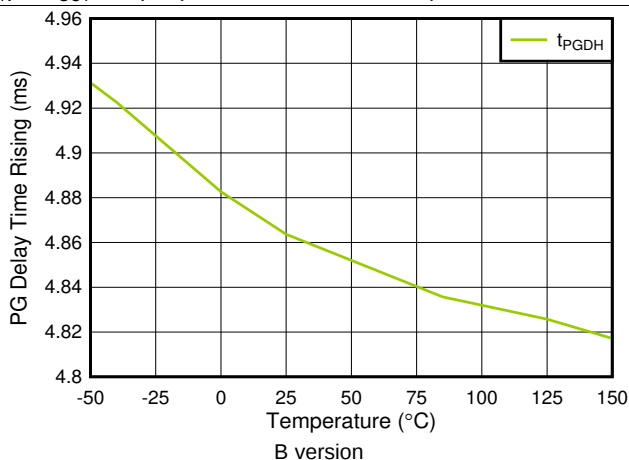
Figure 25. t_{PGDH} vs Temperature (For TPS746B Only)
