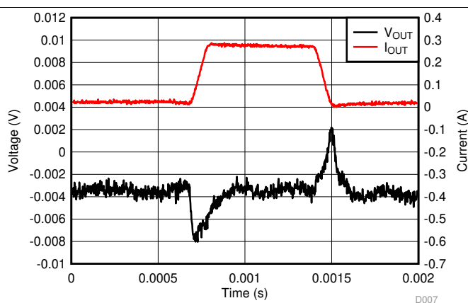
Figure 64. Load Transient
