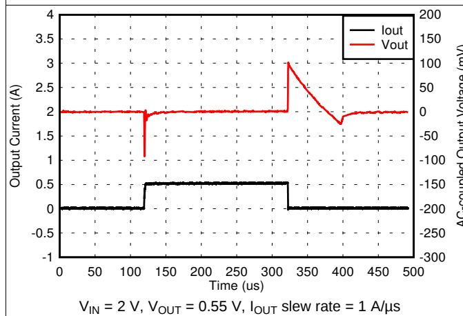
Figure 33. 0.55-V, 1-mA to 500-mA Load Transient
