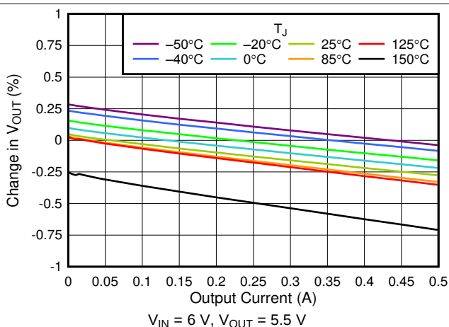
Figure 18. 5.5-V Load Regulation vs I_{OUT}
