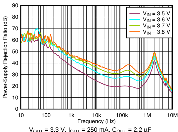
Figure 39. PSRR vs Frequency and V_{IN}
