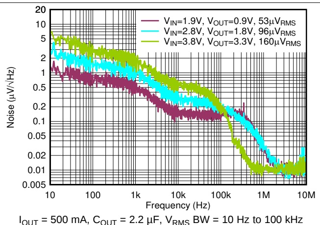
Figure 48. Output Spectral Noise Density vs Frequency
