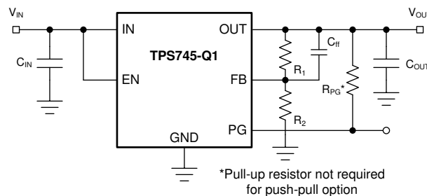
Figure 54. Adjustable Operation
