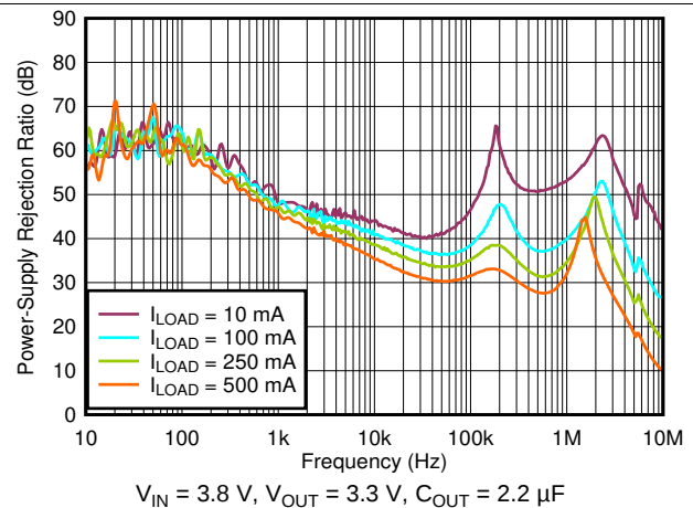
Figure 44. PSRR vs Frequency and I_{LOAD}
