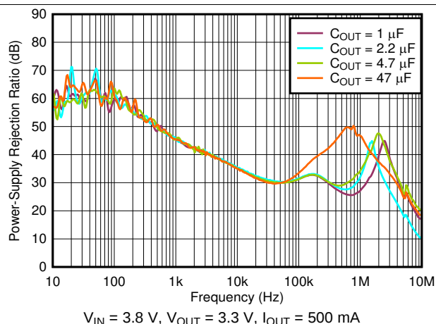
Figure 42. PSRR vs Frequency and C_{OUT}
