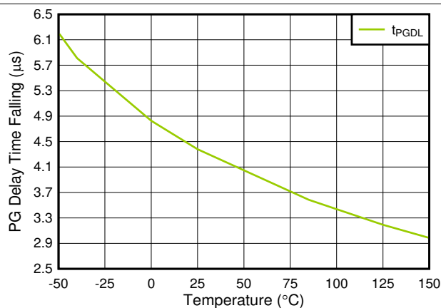
Figure 26. t_{PGDL} vs Temperature
