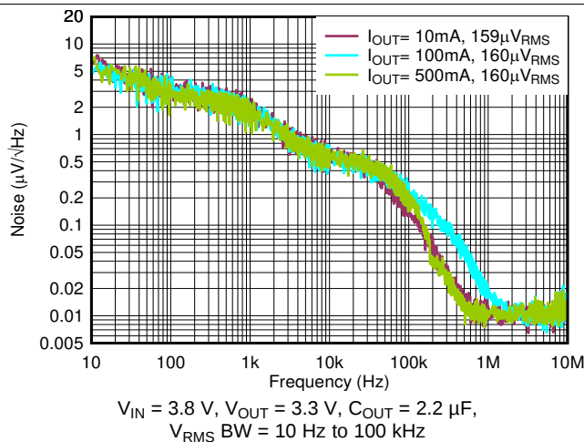
Figure 45. Output Spectral Noise Density vs Frequency and I_{OUT}
