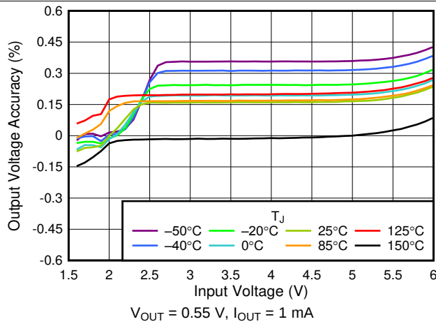
Figure 7. 0.55-V Line Regulation vs V_{IN}
