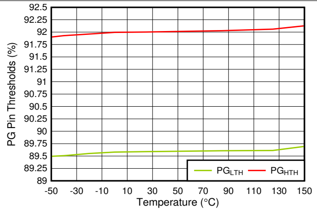
Figure 20. PG_{LTH} and PG_{HTH} vs Temperature
