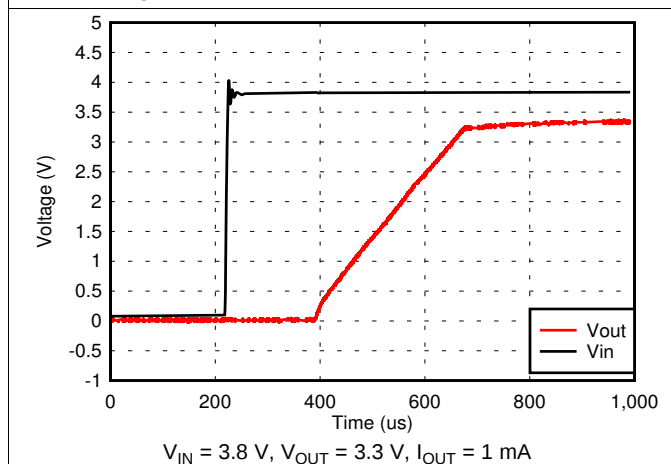
Figure 35. V_{IN} Power-Up
