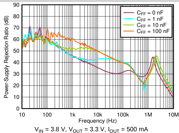
Figure 43. PSRR vs Frequency and C_{FF}
