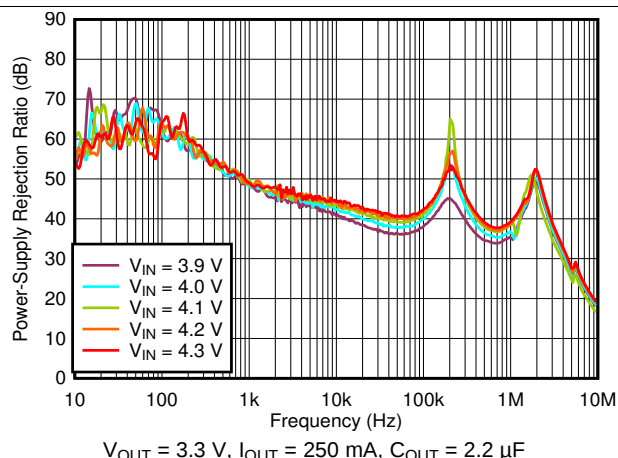
Figure 40. PSRR vs Frequency and V_{IN}
