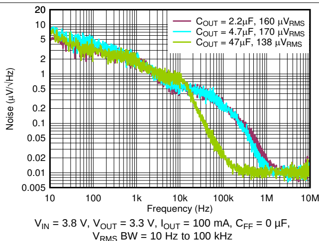
Figure 47. Output Spectral Noise Density vs Frequency and C_{OUT}
