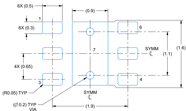
LAND PATTERN EXAMPLE EXPOSED METAL SHOWN SCALE:25X
