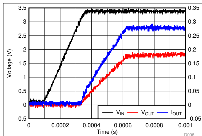
Figure 63. Startup
