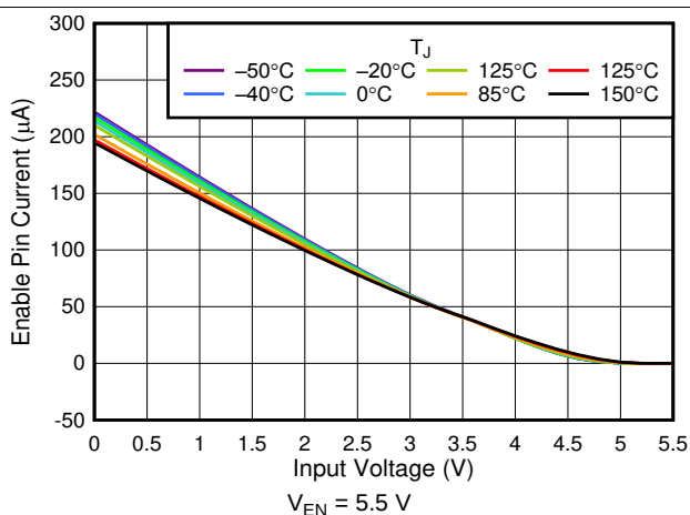
Figure 28. I_{EN} vs V_{IN}
