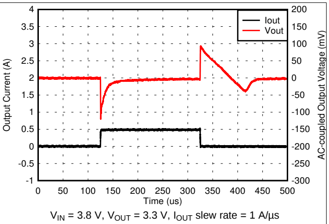
Figure 32. 3.3-V, 1-mA to 500-mA Load Transient
