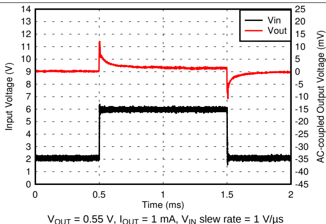
Figure 30. 0.55-V Line Transient
