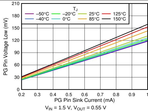
Figure 23. V_{OL(PG)} vs PG Pin Sink Current
