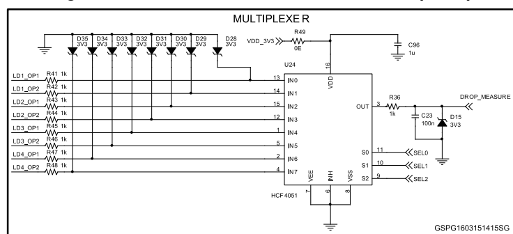
Figure 5: STEVAL-ILL071V1 circuit schematic (5 of 6)
