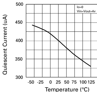
Quiescent Current v Temperature
