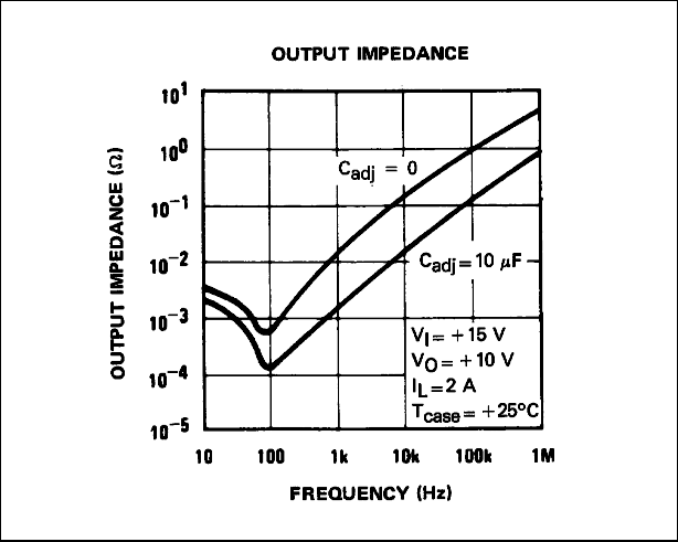
Figure 10. Output impedance
