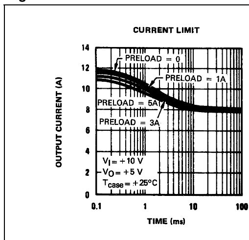
Figure 5. Current limit
