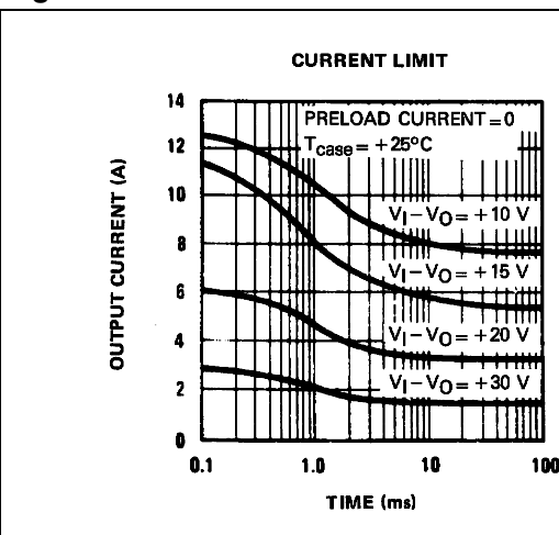
Figure 4. Current limit
