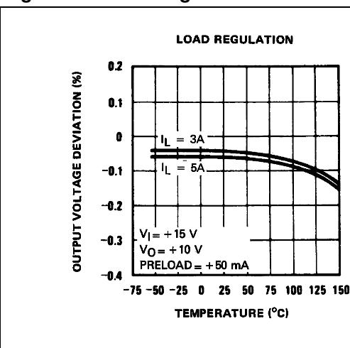
Figure 6. Load regulation
