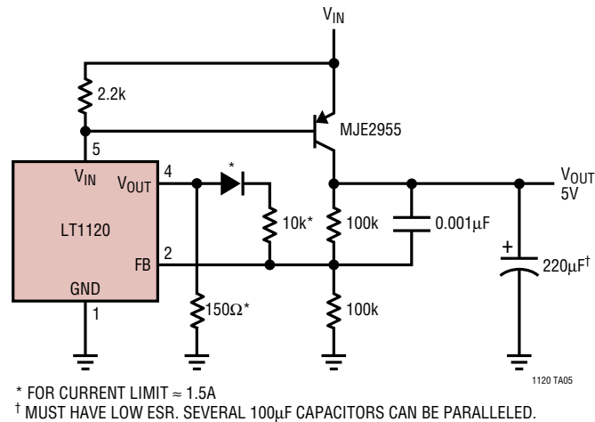
1A Low Dropout Regulator
