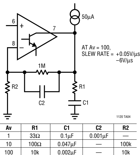
Compensating the Comparator as an Op Amp
