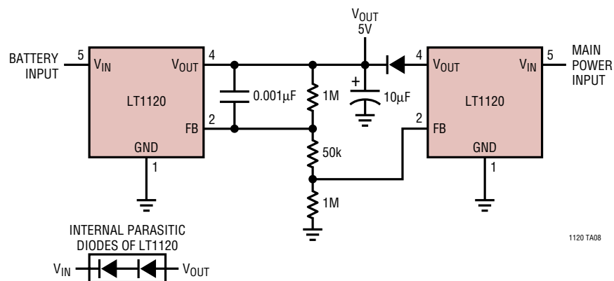
Battery-Backup Regulator
