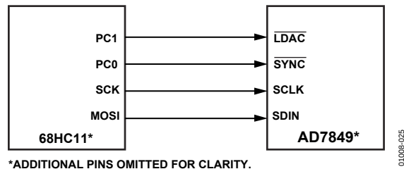
Figure 26. AD7849-to-68HC11 Interface
