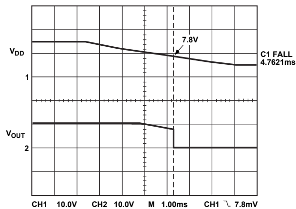
Figure 13. Turn-Off Characteristics
