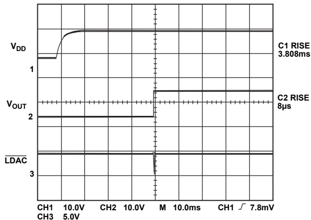
Figure 12. Turn-On Characteristics
