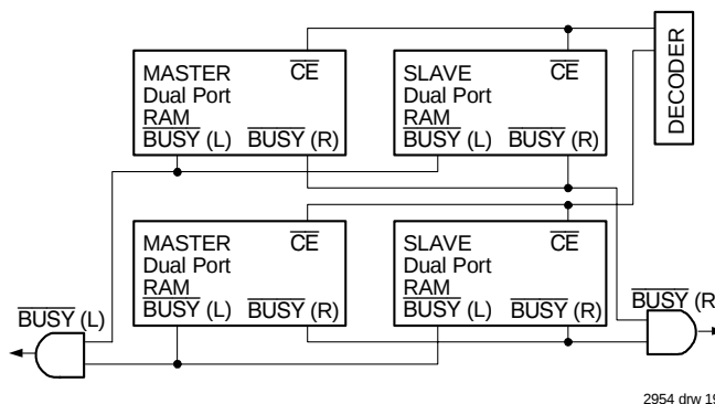
Figure 3. Busy and chip enable routing for both width and depth expansion with IDT7015 RAMs.
