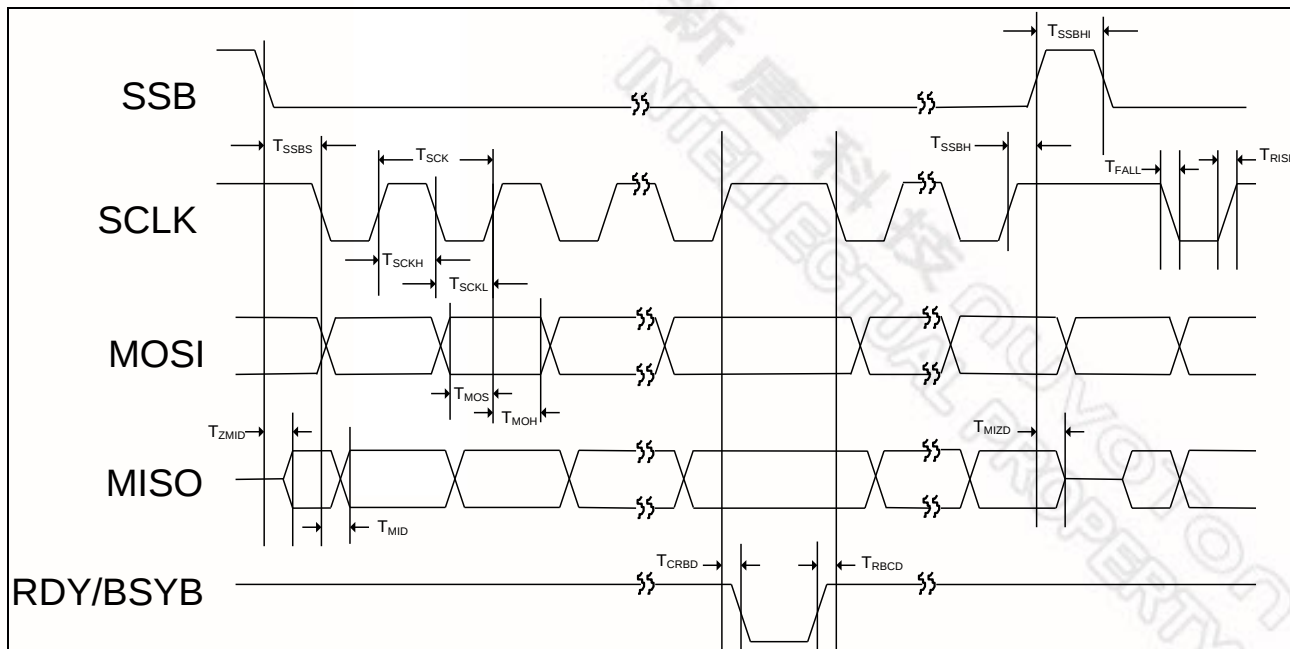
Figure 11-1 SPI Timing
