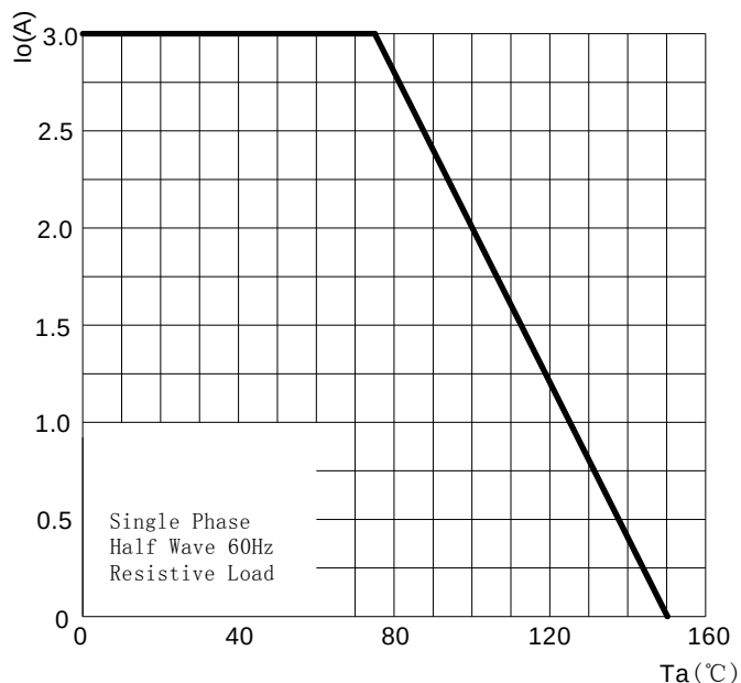
FIG1: Forward Current Dearting Curve
