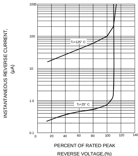
FIG.4-TYPICAL REVERSE CHARACTERISTICS
