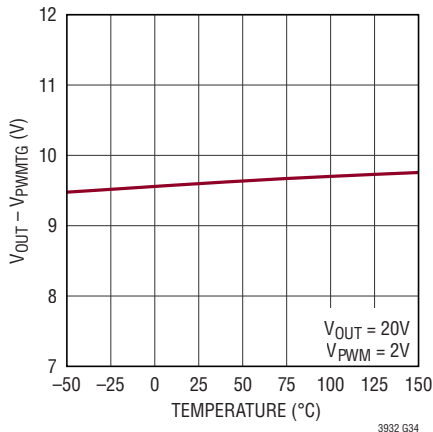
PWMTG Voltage
