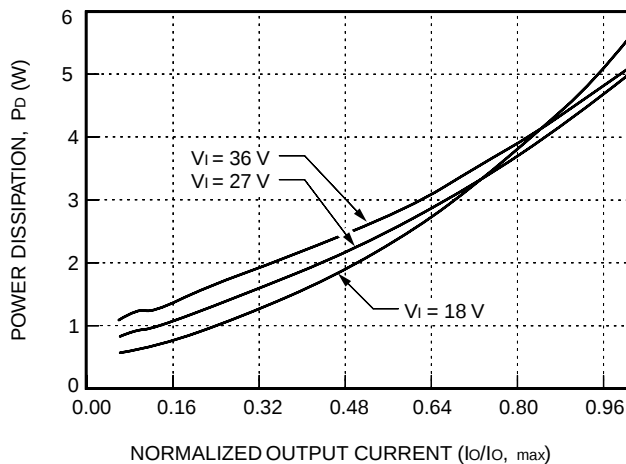
Figure 47. LC015B, C Typical Power Dissipation vs. Normalized Output Current at T_c = 25 °C
