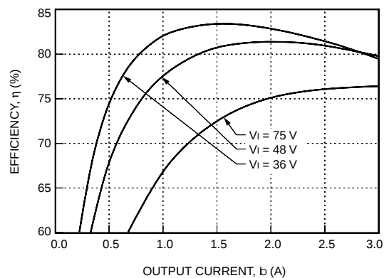
Figure 25. LW015F Typical Efficiency vs. Output Current at T_c = 25^\circ\text{C}
