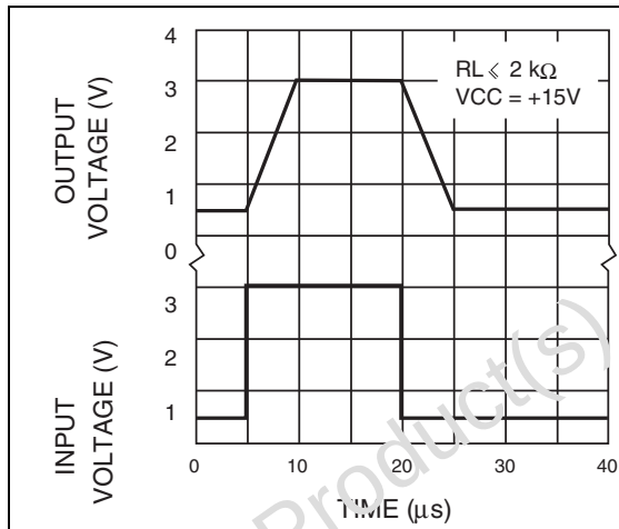
Figure 5. Voltage follower pulse response
