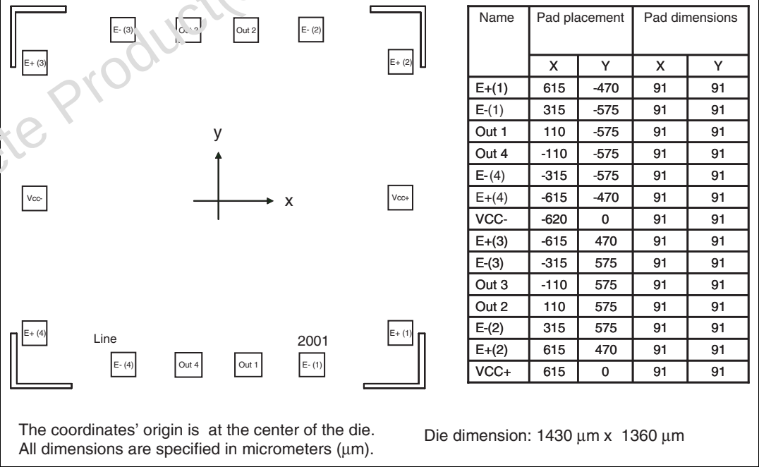
Figure 2. Pad locations
