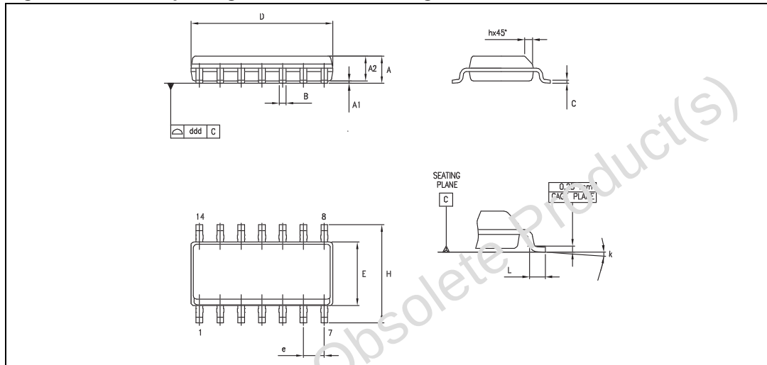
Figure 18. SO-14 package mechanical drawing
