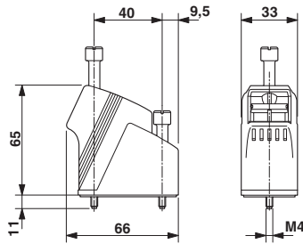
Dimensioned drawing
