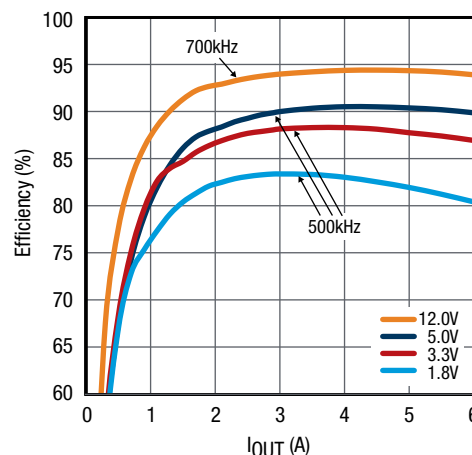
Figure 2. Efficiency, 24VIN
