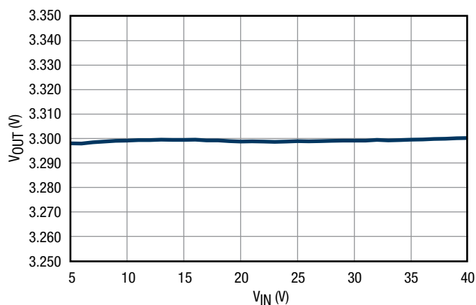
Figure 4. Line Regulation
