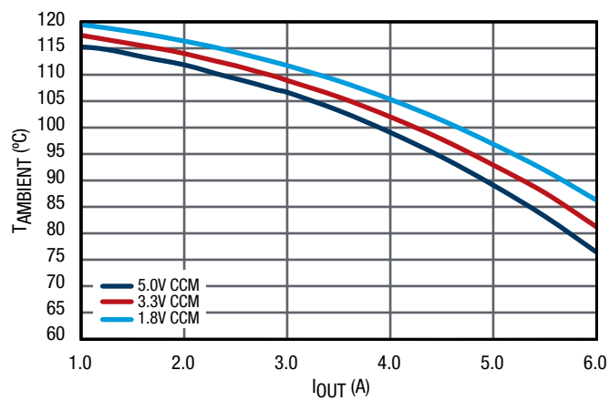
Figure 21. Maximum T_{AMBIENT} vs. I_{OUT} , V_{IN} = 12\text{V}
