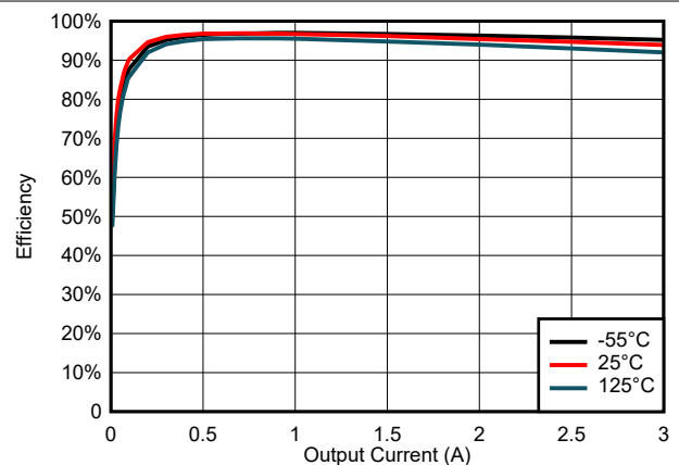
Figure 6-32. Efficiency for V_{\text{IN}} = 5 \text{ V}
