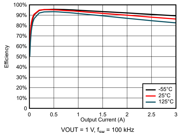
Figure 6-16. Efficiency for VIN = 3 V
