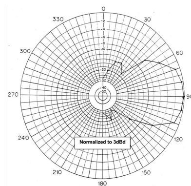
Azimuthal Pattern (Y, Z, or E-plane)
