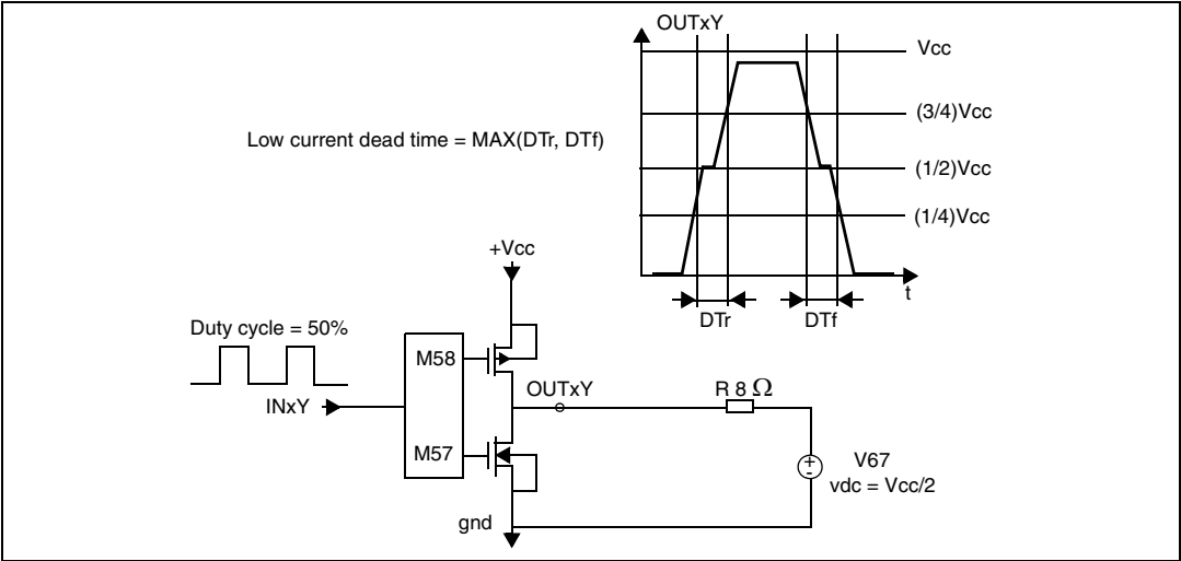
Figure 5. Test circuit 1
