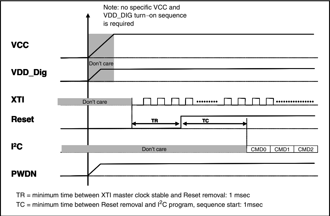
Figure 3. Power-on sequence
