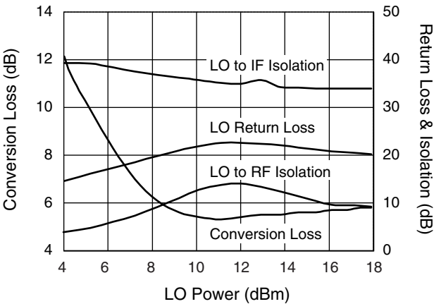
Performance vs. LO Power F_{RF} = 28\text{ GHz} , F_{LO} = 27\text{ GHz} , P_{RF} = -10\text{ dBm}
