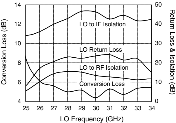
Performance vs. LO Frequency F_{RF} = F_{LO} + 1\text{ GHz} , P_{RF} = 10\text{ dBm}
