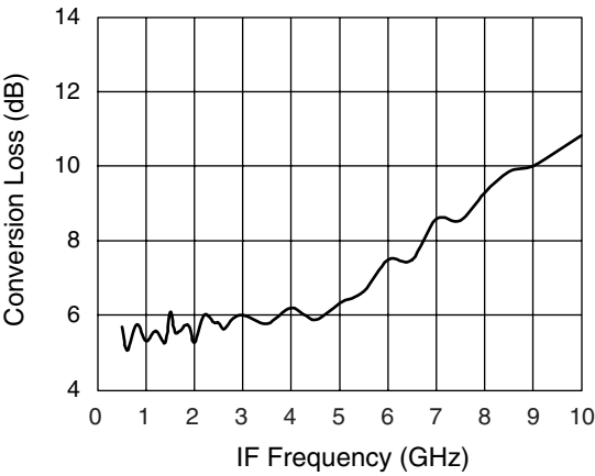
Performance vs. IF Frequency F_{RF} = 28\text{ GHz} , F_{LO} = F_{RF} + F_{IF} , P_{LO} = 10\text{ dBm}
