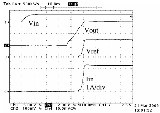
Figure 10. Start up V_{in}=3.3V , I_{out}=1.5A
