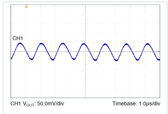
Figure 81 — Output Voltage Ripple: Nominal Line, Nominal Trim, 50% load, C OUT = 8 x 10μF Ceramic
