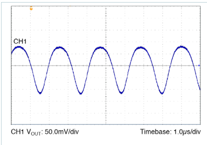
Figure 78 — Output Voltage Ripple: Nominal Line, Nominal Trim, 100% load, C OUT = 8 x 10μF Ceramic
