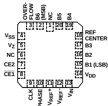
CA3306 (CLCC) TOP VIEW
