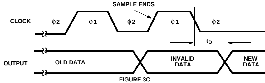
FIGURE 3. PULSE MODE
