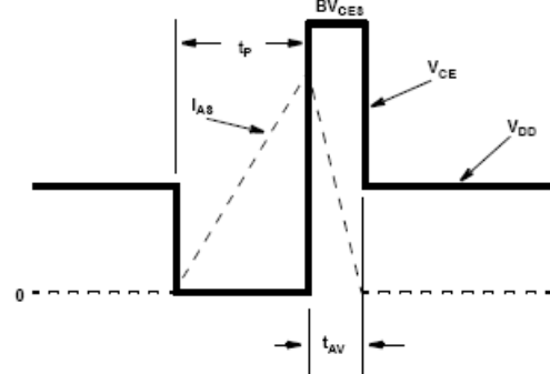
Figure 20. Energy Waveforms
