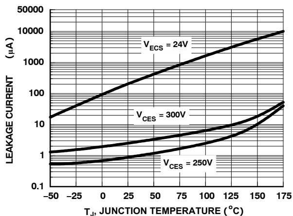
Figure 11. Leakage Current vs. Junction Temperature
