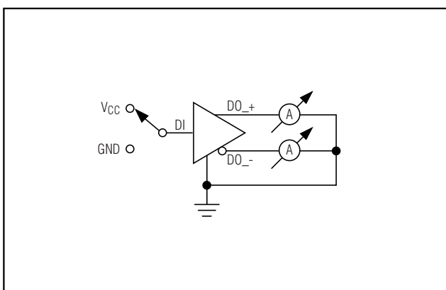
Figure 6. Short-Circuit Measurements
