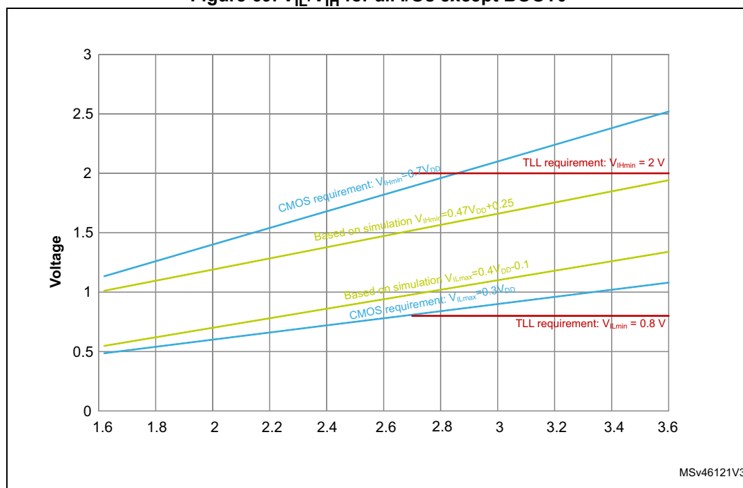
Figure 69. V_{IL}/V_{IH} for all I/Os except BOOT0
