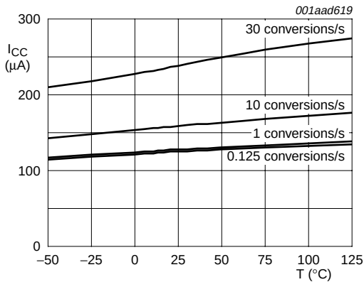
Fig 14. Typical normal I²C-bus inactive supply current as a function of temperature
