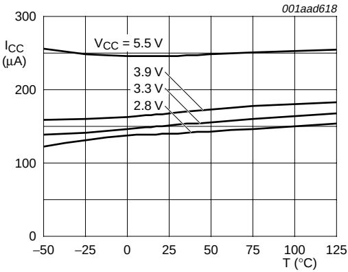
Fig 13. Typical normal I²C-bus inactive supply current as a function of temperature
