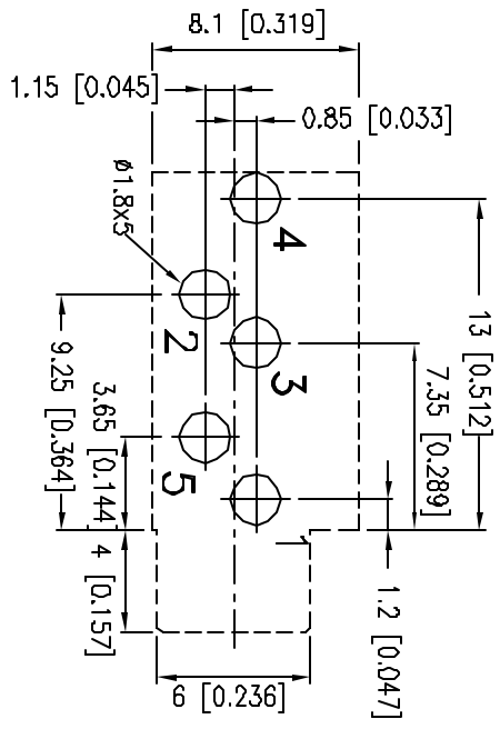
HOLE LAYOUT (TOP VIEW)
