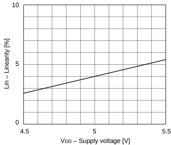
Linearity vs. Supply voltage
