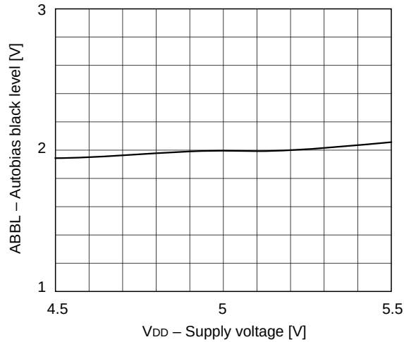
Autobias black level vs. Supply voltage
