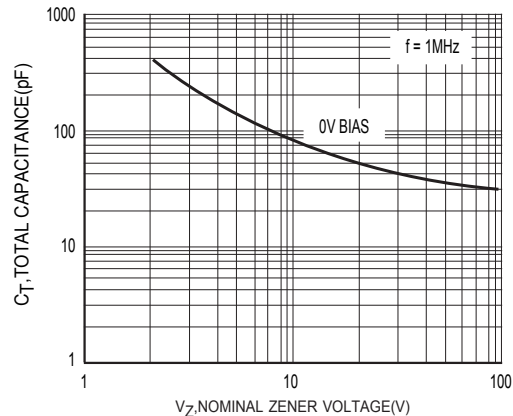
Figure 2 Typical Capacitance
