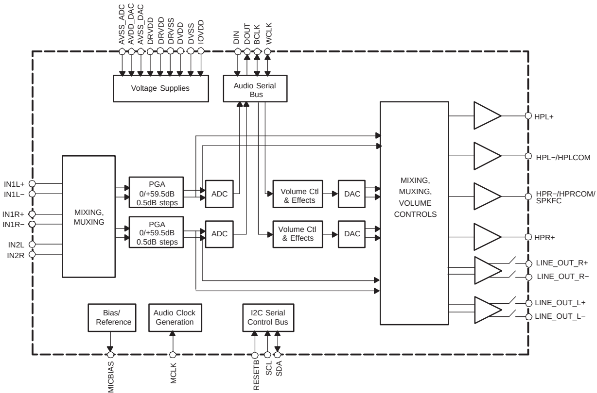
Figure 1. Simplified Codec Block Diagram
