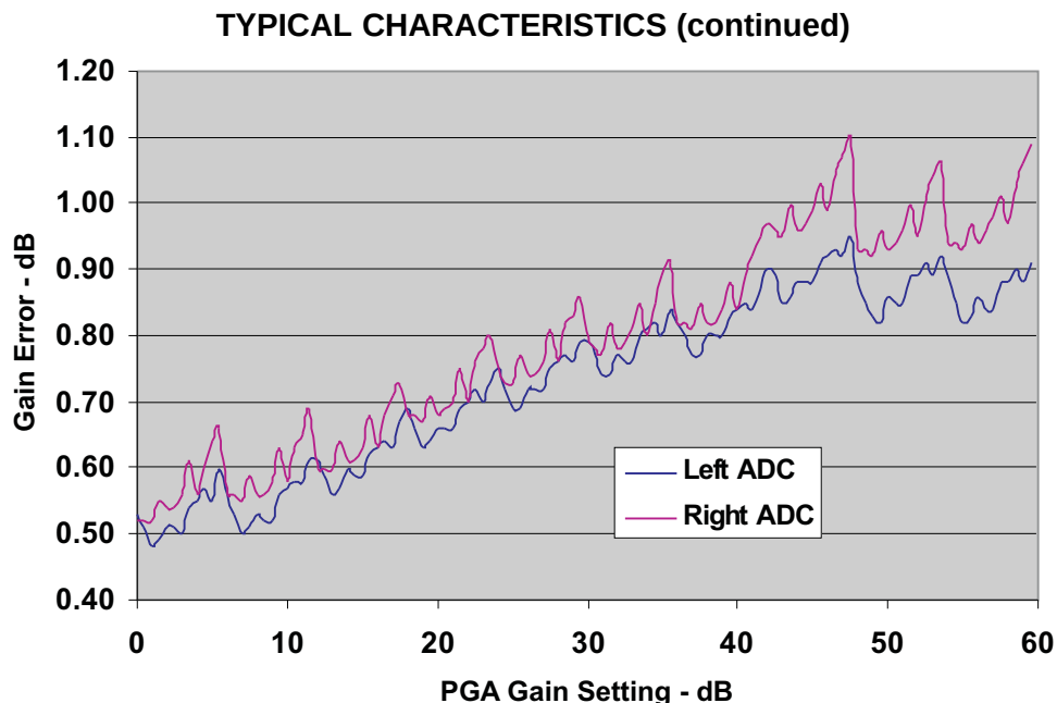
Figure 12. ADC Gain Error vs PGA Gain Setting
