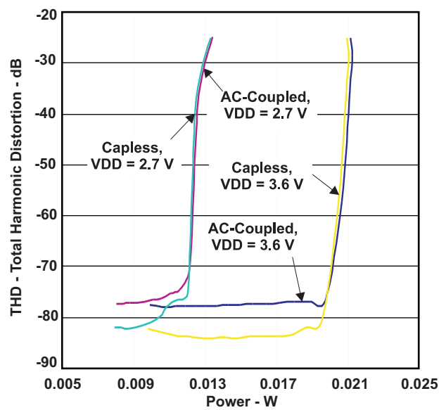
Figure 7. Headphone Power vs THD, 32 \Omega Load
