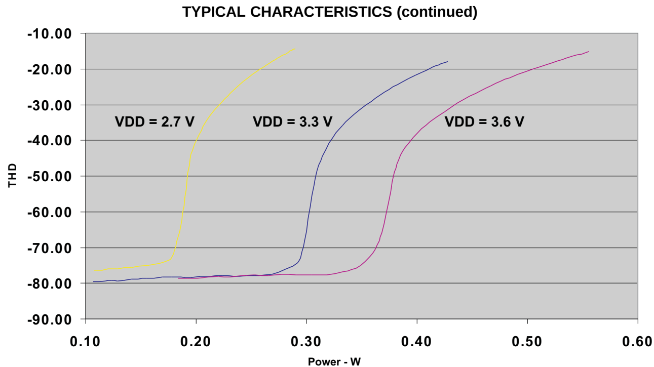
Figure 10. Speaker Power vs THD, 8 \Omega Load
