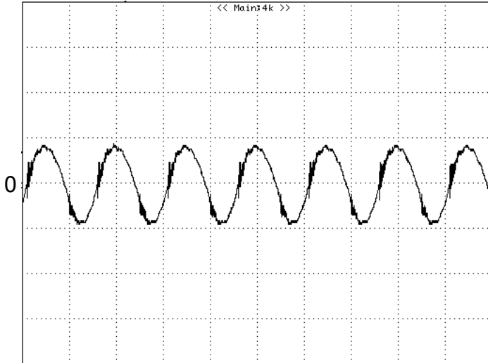
Figure 11: Input Terminal Ripple Current, i_c , at full rated output current and nominal input voltage with 12\mu\text{H} source impedance and 33\mu\text{F} electrolytic capacitor (500 mA/div, 2 \mu\text{s} /div)
