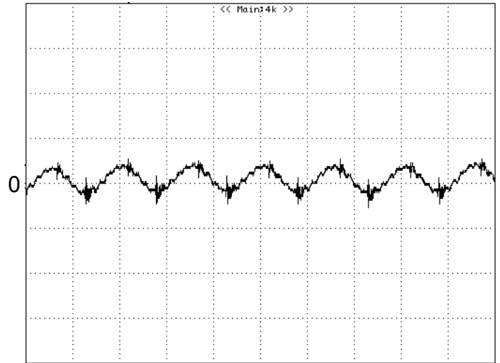
Figure 12: Input reflected ripple current, i_s , through a 12\mu\text{H} source inductor at nominal input voltage and rated load current (20 mA/div, 2 \mu\text{s} /div)
