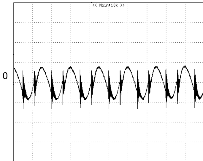
Figure 14: Output voltage ripple at nominal input voltage and rated load current ( I_o=25A ) (10 mV/div, 2 μs/div) Load capacitance: 1 μF ceramic capacitor and 10 μF tantalum capacitor. Bandwidth: 20 MHz. Scope measurements should be made using a BNC cable (length shorter than 20 inches). Position the load between 51 mm to 76 mm (2 inches to 3 inches) from the module
