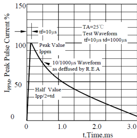
Fig. 3-Pulse Waveform
