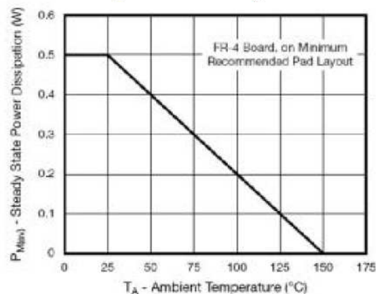
Fig. 2-Power Derating Curve
