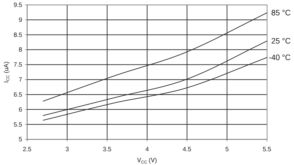
Figure 27-9. ATmega8U2: Power-Down Supply Current vs. V_{CC} (Watchdog Timer Enabled)
