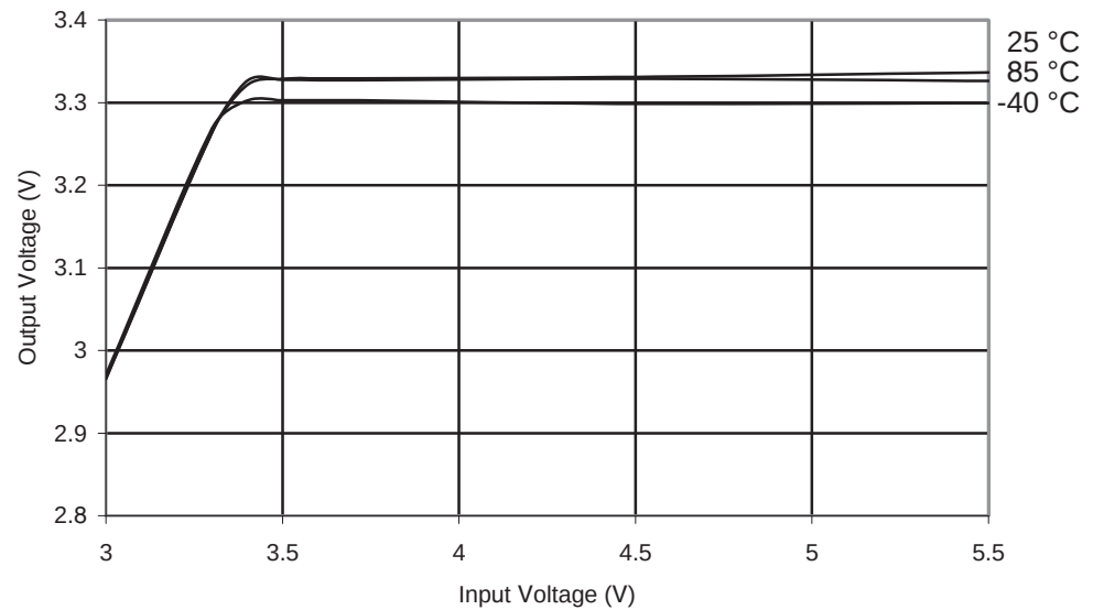
Figure 27-37. ATmega8U2: USB Regulator Level vs. V_{CC}
