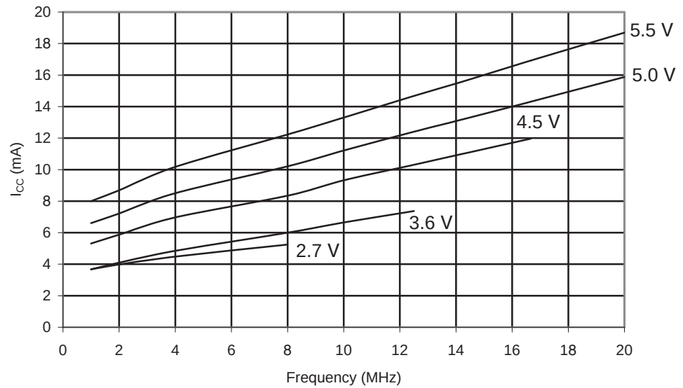
Figure 27-3. ATmega8U2: Active Supply Current vs. Frequency (1-20 MHz) and T = 25^{\circ}\text{C}
