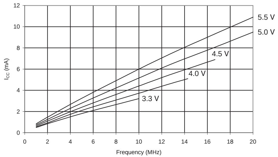
Figure 27-7. ATmega8U2: Idle Supply Current vs. Frequency (1-20 MHz) T = 85^{\circ}\text{C}
