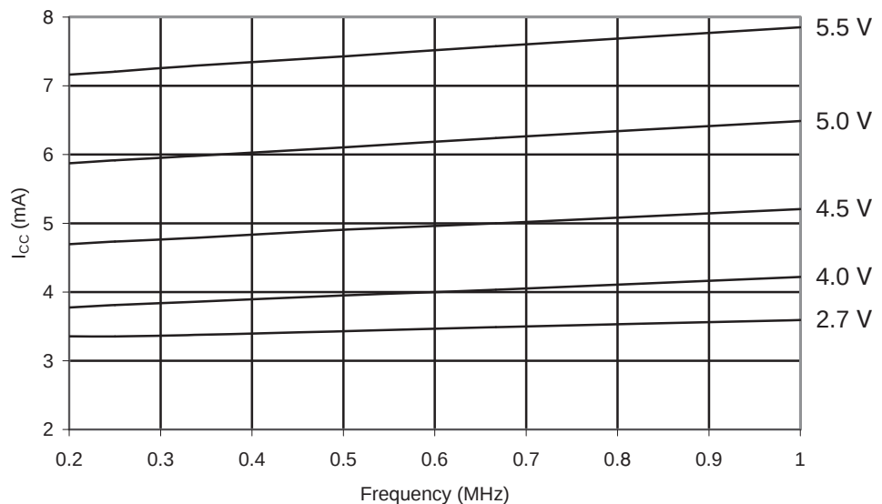
Figure 27-1. ATmega8U2: Active Supply Current vs. Low Frequency (1MHz) and T = 25^\circ\text{C}
