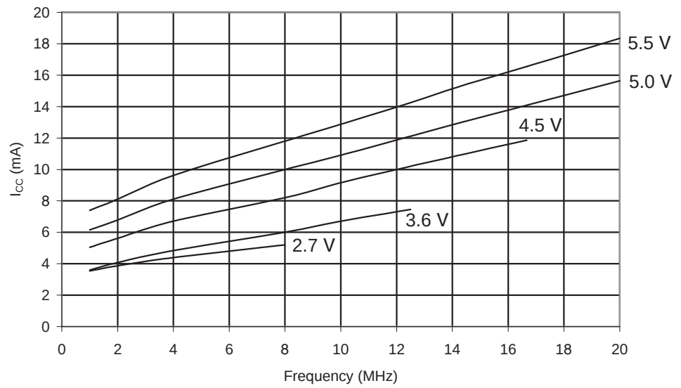
Figure 27-4. ATmega8U2: Active Supply Current vs. Frequency (1-20 MHz) and T = 85^{\circ}\text{C}
