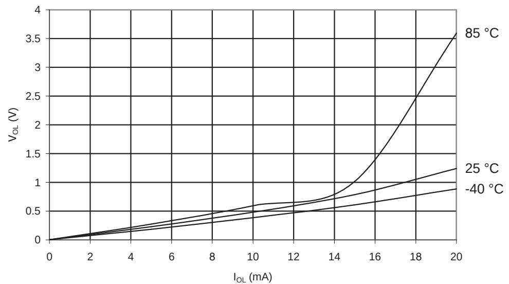
Figure 27-15. ATmega8U2: I/O Pin Output Voltage vs. Sink Current ( V_{CC} = 5\text{ V} )
