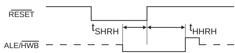
Figure 26-4. Hardware Boot Timing Requirements
