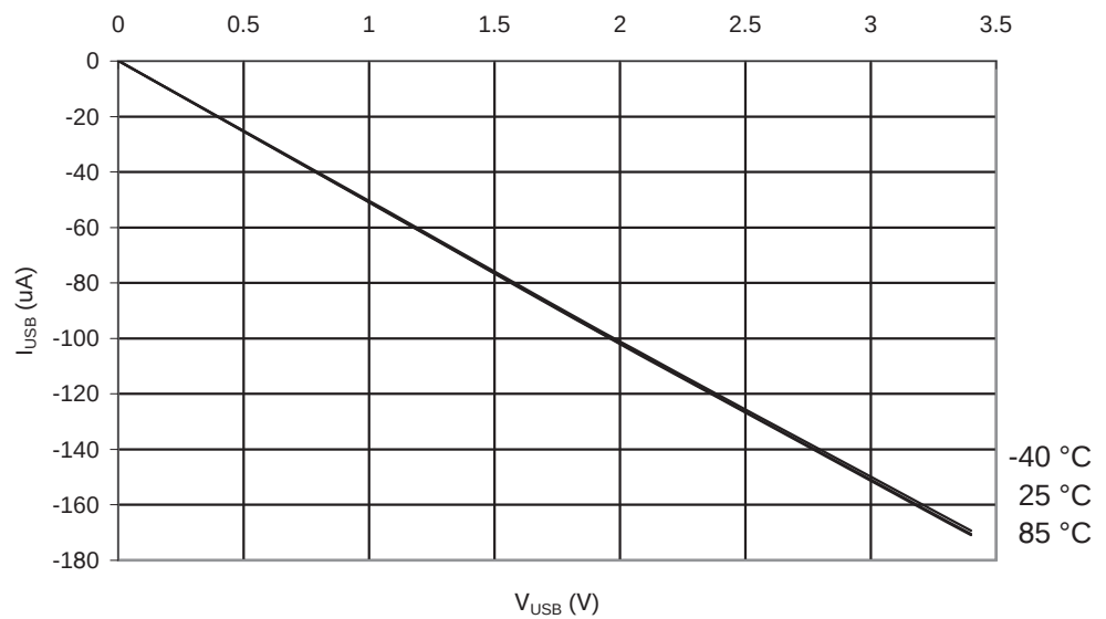
Figure 27-19. ATmega8U2: USB DP HI Pull-Down Resistor Current vs. USB Pin Voltage
