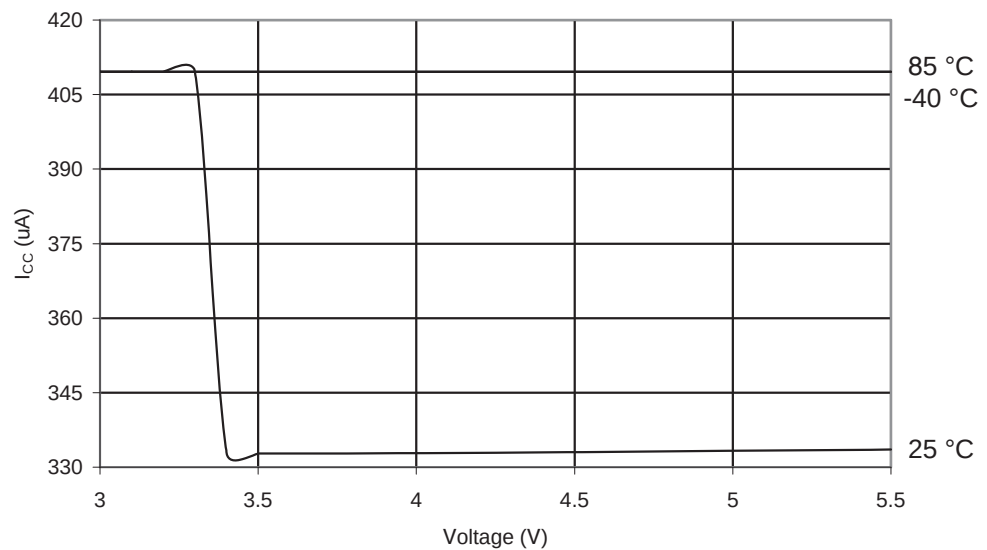
Figure 27-35. ATmega8U2: USB Regulator Consumption vs. V_{CC}
