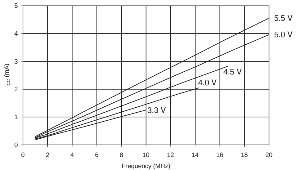
Figure 27-6. ATmega8U2: Idle Supply Current vs. Frequency (1-20 MHz) T = 25^{\circ}\text{C}
