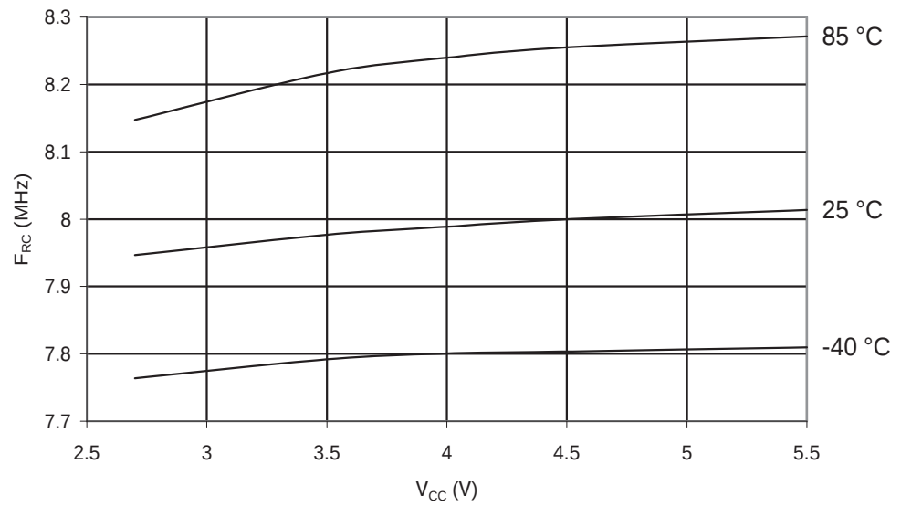
Figure 27-32. ATmega8U2: Calibrated 8 MHz RC Oscillator Frequency vs. V_{CC}
