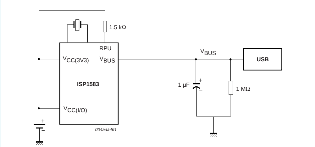
Fig 14. Self-powered mode.
