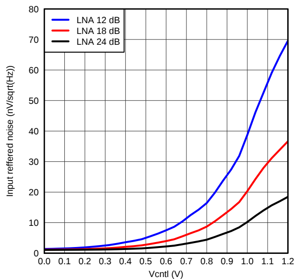
Figure 22. IRN, PGA = 24dB and Low Power Mode
