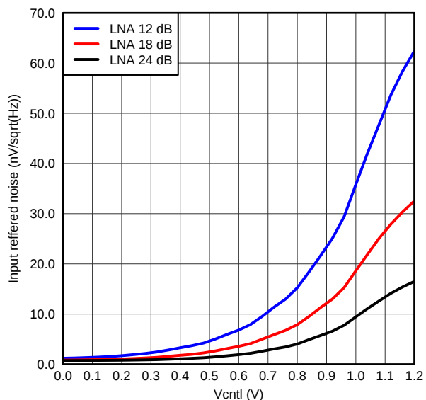
Figure 18. IRN, PGA = 24dB and Low Noise Mode
