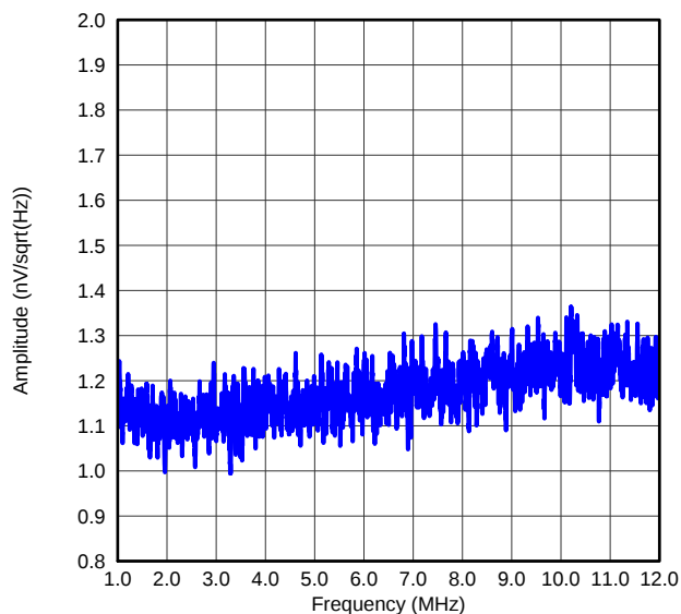
Figure 27. IRN, PGA = 24dB and Low Power Mode
