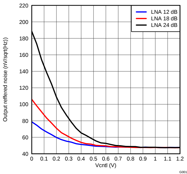
Figure 24. ORN, PGA = 24dB and Low Noise Mode
