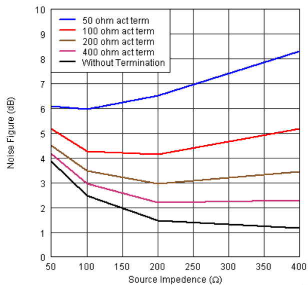
Figure 32. Noise Figure, LNA = 18dB and Low Power Mode
