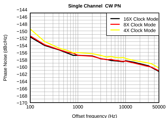
Figure 15. CW Phase Noise, F_{in} = 2\text{MHz}
