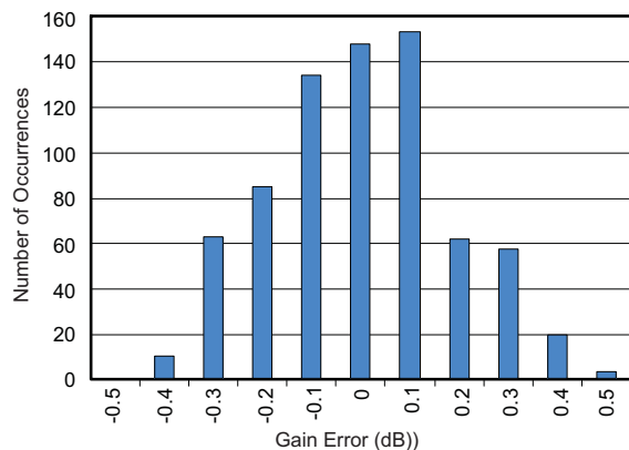
Figure 4. Gain Matching Histogram, V_{CNTL} = 0.3\text{V} (936 Channels)
