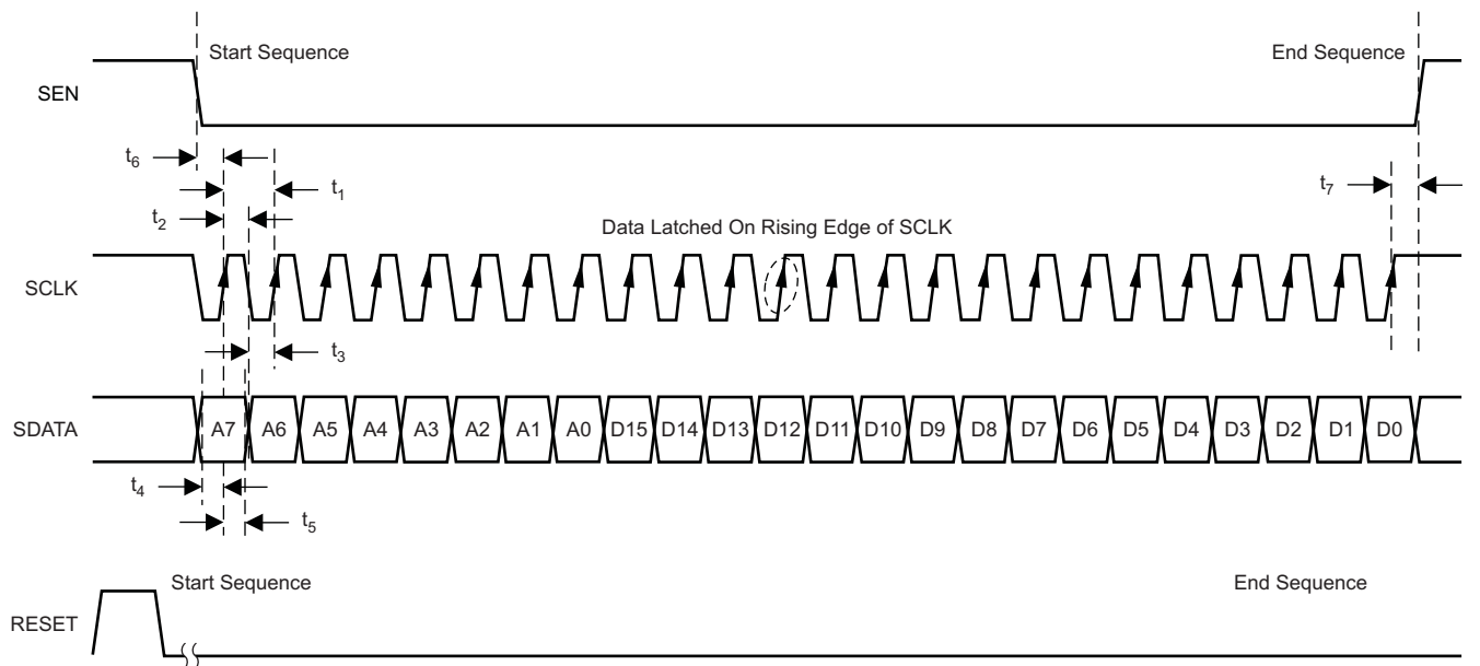
Figure 60. SPI Timing
