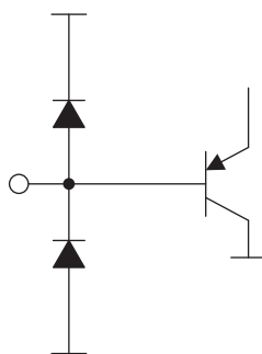
Figure 78. Equivalent Circuits of V_{\text{CNTLP/M}}
