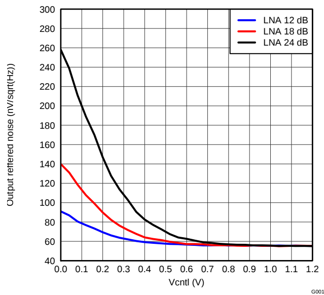
Figure 25. ORN, PGA = 24 dB and Medium Power Mode
