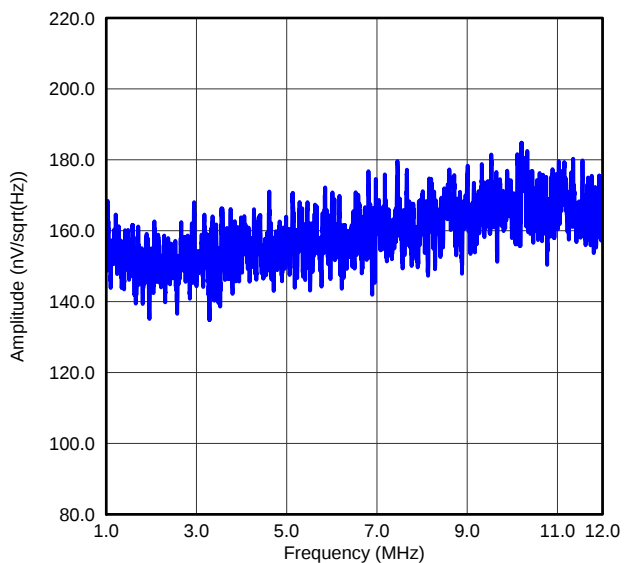
Figure 28. ORN, PGA = 24dB and Low Power Mode
