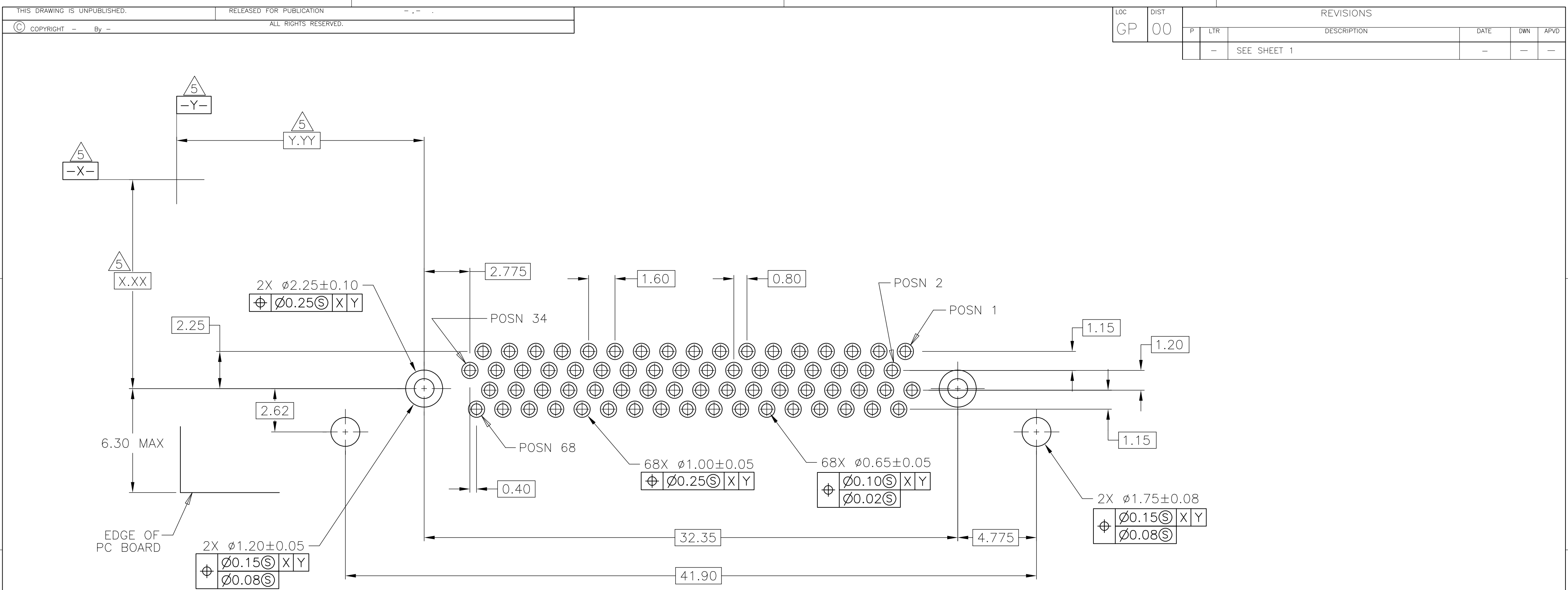
PC BOARD MOUNTING DIMENSIONS
