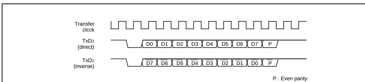
Figure 2.11.29 SIM interface format
