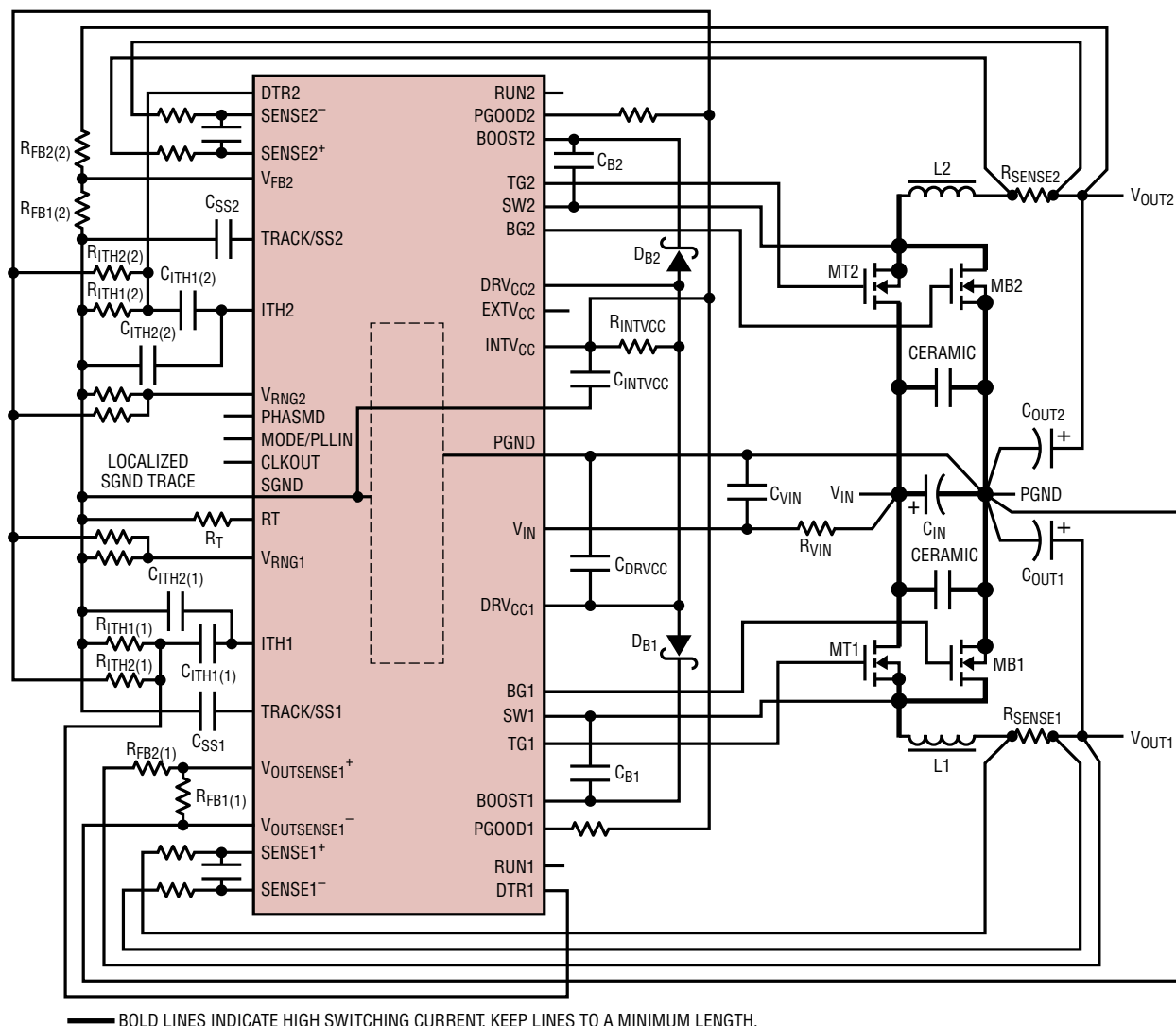
Figure 14. Recommended PCB Layout Diagram
