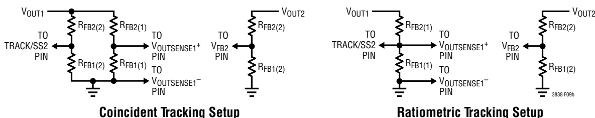
Figure 9b. Setup for Coincident and Ratiometric Tracking
