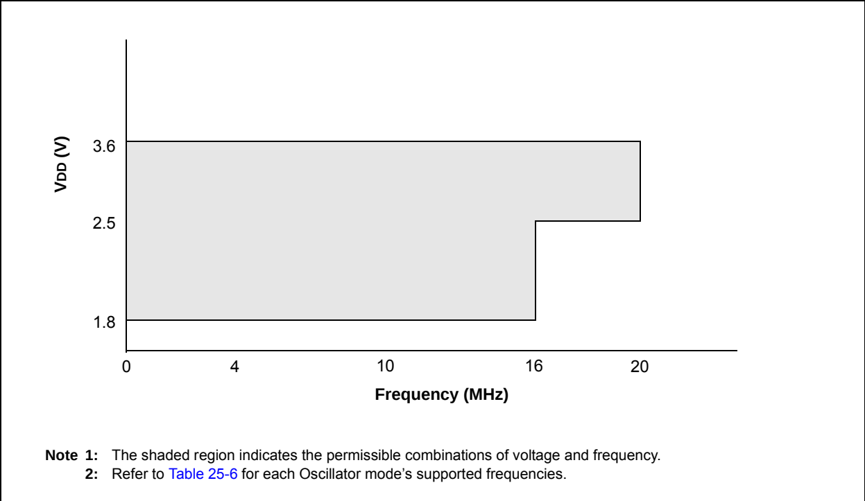
FIGURE 25-2: PIC16LF1512/3 VOLTAGE FREQUENCY GRAPH, -40°C ≤ TA ≤ +125°C
