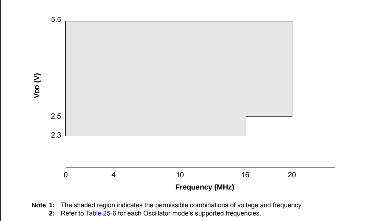
FIGURE 25-1: PIC16F1512/3 VOLTAGE FREQUENCY GRAPH, -40°C ≤ TA ≤ +125°C
