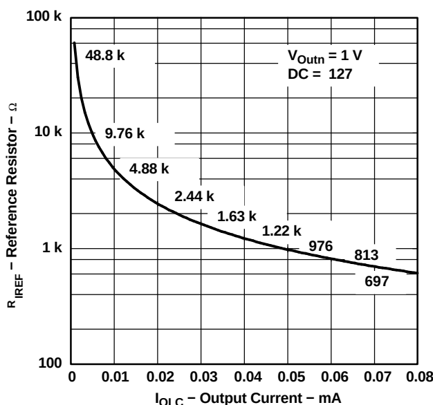
Figure 8. Reference Resistor vs Output Current
