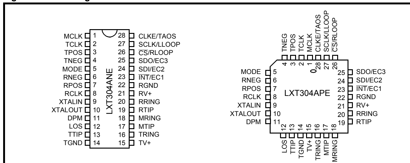
Figure 1: Pin Assignments
