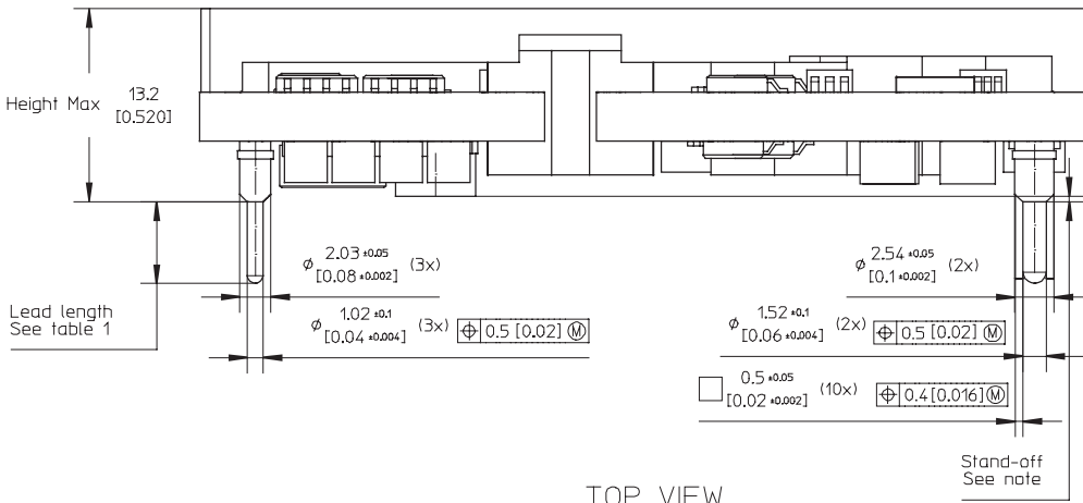
Pin positions according to recommended footprint
