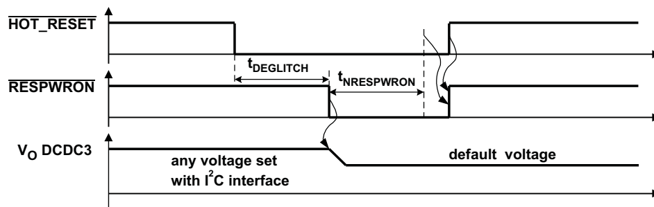
Figure 26. HOT_RESET Timing
