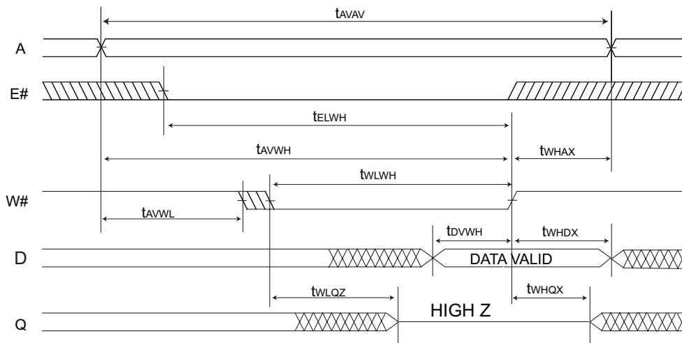
FIGURE 4 – WRITE CYCLE 1 - W# CONTROLLED
