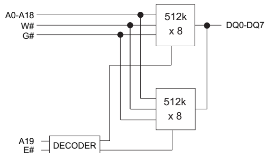
Block Diagram
