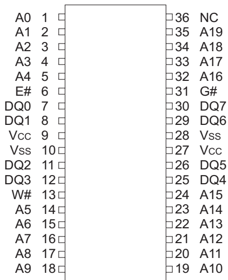
Pin Configuration
