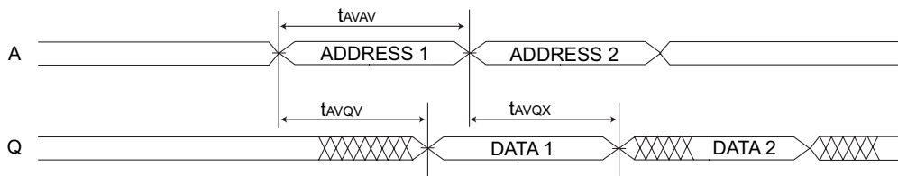
FIGURE 2 – READ CYCLE 1 - W# HIGH, G#, E# LOW
