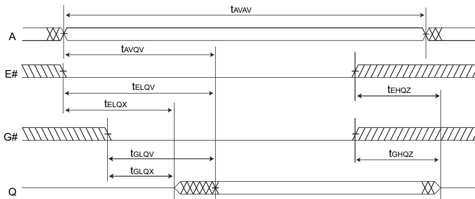
FIGURE 3 – READ CYCLE 2 - W# HIGH
